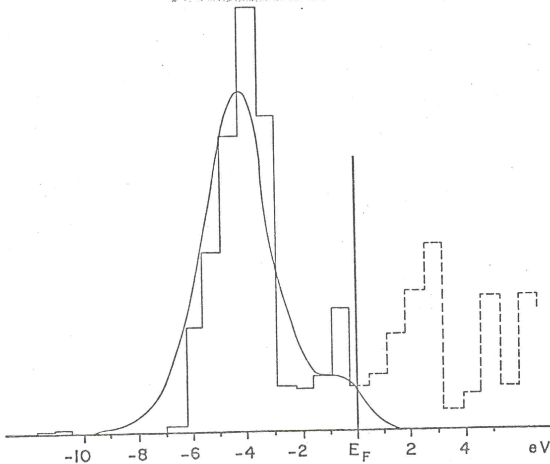
FIG. 14. C-K emission from NbC .
